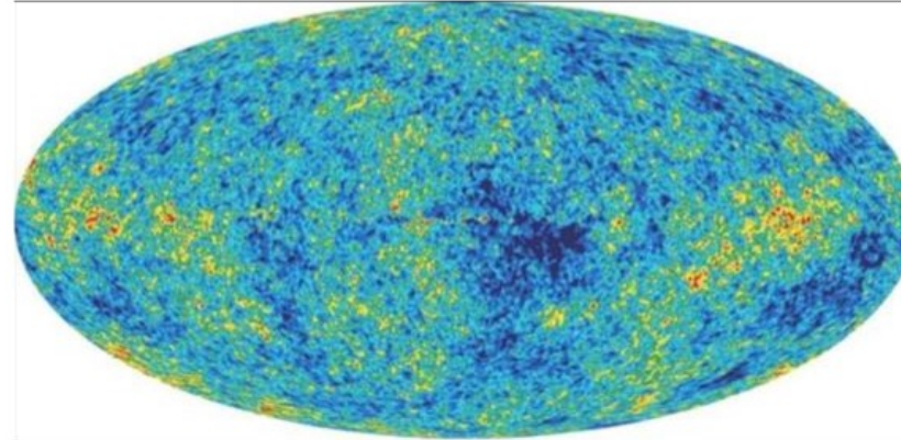
WMAP (2003)
