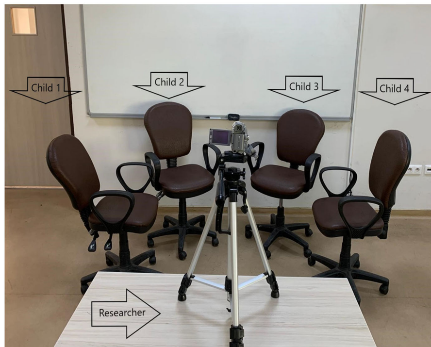
Figure 1. Demonstration of the game setting. Note. The game setting was identical in the cooperative and solitary versions.
